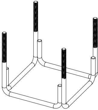
Fig. 1: Prefabricated anchor
