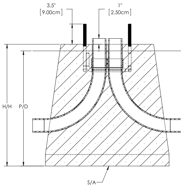
Fig. 3: Concrete Base
