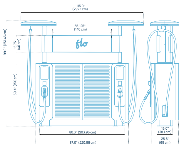
Pull-in configuration
