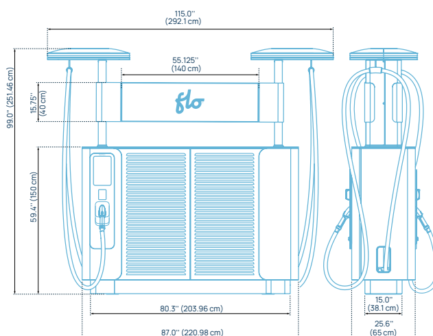
Pull-through configuration
